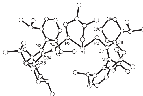
Figure 2. Solid-state structure of 3 (hydrogen atoms have been omitted for clarity). Selected bond lengths [Å] and angles [ ^\circ ]: P1–P2 2.227(3), P1–P3 2.236(3), P2–P4 2.226(3), P4–C7 1.744(7), P3–C34 1.730(8), N1–C34 1.379(10), N2–C7 1.363(9); C7–P4–P2 114.3(3) , C34–P3–P1 110.1(3) , P2–P1–P3 94.21(10) , P4–P2–P1 92.55(10) , N1–C34–C35 108.3(6) , N2–C7–C8 109.4(6) .
